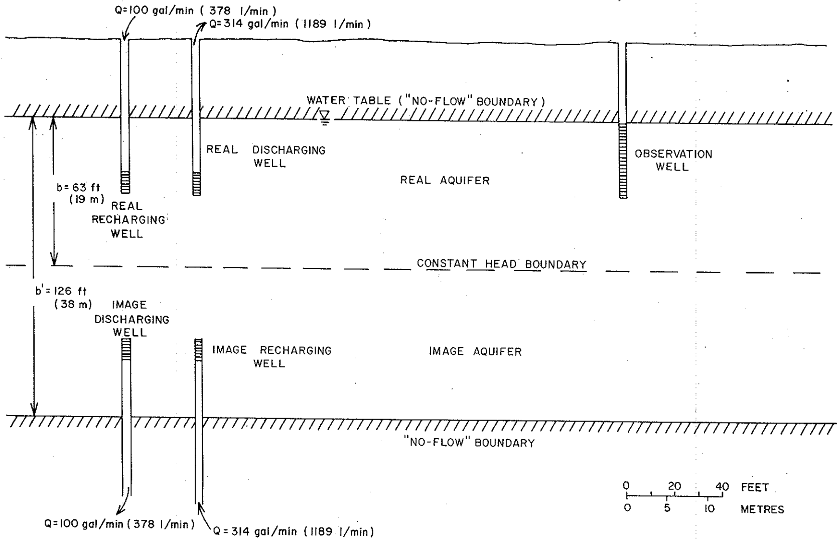
FIGURE 6.--SKETCH SHOWING BOUNDARY CONDITIONS AND CONCEPTUAL MODEL USED IN ANALYSIS OF DATA FROM AQUIFER TEST 1.
