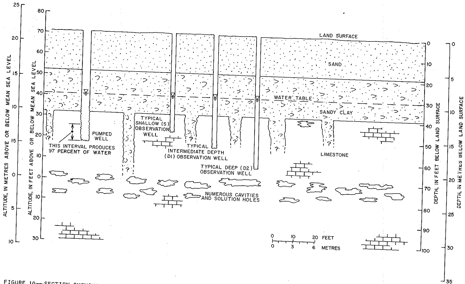
FIGURE 10.—SECTION SHOWING GENERALIZED GEOLOGY AND WELL CONSTRUCTION OF PUMPED WELL AND TYPICAL OBSERVATION WELLS AT AQUIFER TEST SITE 2.
